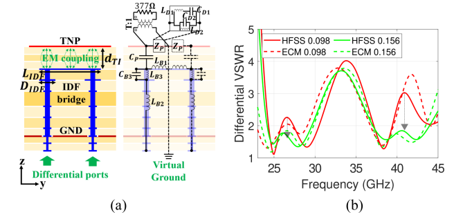
Fig. 5. (a) Illustration of the EM coupling between the TNP antenna and the IDF bridge, along with the corresponding equivalent circuit model. The optimized circuit parameter values are as follows: ( L_{B1} , L_{B2} , L_{B3} , R_{LB2} , R_{LB3} , L_{D1} , L_{D2} , C_P , C_{B3} , C_{D1} , C_{D2} , T ) = (14, 0.6, 0.12, 9.3, 3.56, 9.3, 0.30, 0.052, 41.9, 190.4, 72.9, 518.9, 0.364) where the units are nH, \Omega , and fF, respectively. (b) Differential VSWR results obtained from HFSS and equivalent circuit simulations for varying d_{TI} (in mm). The case with d_{TI} = 0.156 corresponds to the optimized configuration, whereas d_{TI} = 0.098 represents a comparative case with updated circuit parameters: ( L_{B2} , L_{D1} , L_{D2} , C_P , C_{D1} ) = (0.65, 0.196, 0.048, 46.1, 72.9).
