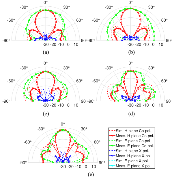
Fig. 10. Simulated (measured) E-plane and H-plane radiation patterns at (a) 24.25 GHz (24.5 GHz), (b) 26.5 GHz (27.0 GHz), (c) 29.5 GHz (29.5 GHz), (d) 37 GHz (37 GHz), and (e) 39.25 GHz (38.5 GHz), respectively.
