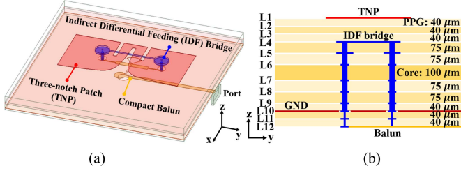
Fig. 1. Illustration of (a) TNP antenna with an IDF bridge and (b) PCB stackup.
