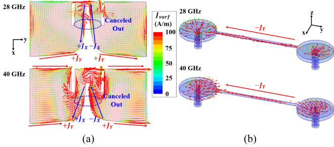
Fig. 3. Surface current distribution on (a) TNP in L1 and (b) IDF bridge in L4.
