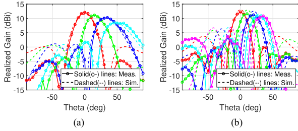
Fig. 11. Simulated (measured) scanned radiation patterns within -3 dB scan range at (a) 26.5 GHz (27 GHz) and (b) 39.25 GHz (38.5 GHz).
