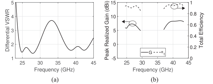
Fig. 6. Simulated (a) differential VSWR, and (b) peak gain and total efficiency versus frequency for the TNP antenna element.
