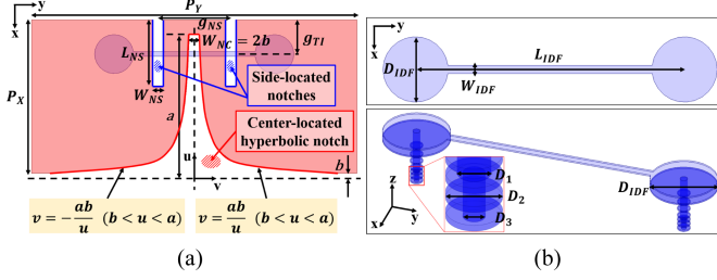
Fig. 2. Design parameters of the proposed antenna components. (a) TNP in L1 with the IDF bridge in L4-L9. The assigned design parameter values (in mm) are P_X = 3.15 , P_Y = 6.7 , L_{NS} = 1.35 , g_{NS} = 1.7 , W_{NS} = 0.2 , W_{NC} = 2b = 0.2 , a = 3 , b = 0.1 , g_{TI} = 0.7 , D_{IDF} = 1 , L_{IDF} = 3.3 , W_{IDF} = 0.1 , D_1 = 0.09 , D_2 = 0.15 , and D_3 = 0.06 .
