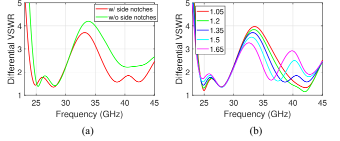
Fig. 4. Simulated differential VSWR. (a) With and without the two side notches, and for a variation in (b) L_{NS} (units: mm).
