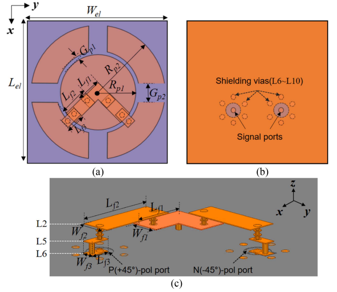
Fig. 3. (a) Top view. (b) Bottom view of proposed antenna. (c) Detailed description of the MUB feeding structure.
