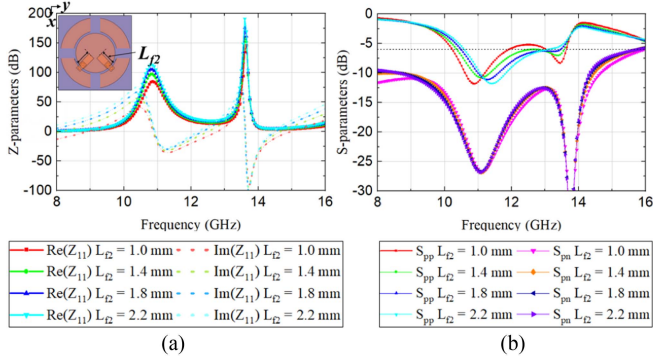
Fig. 4. Proposed antenna with L-probe feeding structure instead of MUB feeding structure. (a) Z-parameters along the variation of L_{f2} . (b) S-parameters along the variation of L_{f2} .
