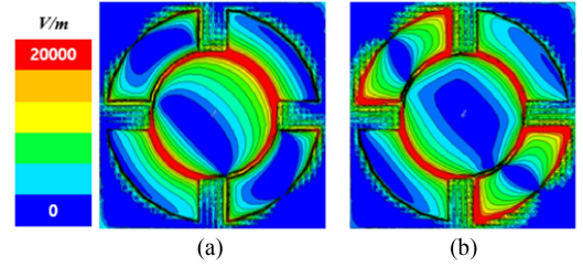
Fig. 7. Electric field distribution of the proposed antenna on the top layer when P-port is ON. (a) 10 GHz. (b) 12.7 GHz.
