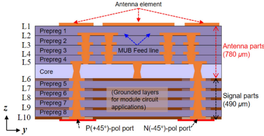
Fig. 2. Layer stack-up of the proposed AoP module: ten layers.
