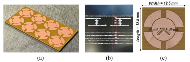
Fig. 9. (a) Fabricated 2 \times 4 antenna array. (b) X-ray photograph of the side cross section of the fabricated sample. (c) Top view of the radiating patch with an added slot structure.
