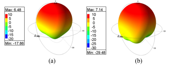
Fig. 8. 3-D far-field radiation pattern of realized gain when P-port is ON. (a) 10 GHz. (b) 12.7 GHz.
