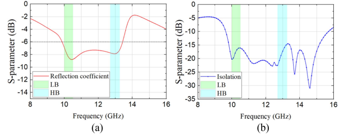
Fig. 6. (a) Reflection coefficient and (b) isolation of the proposed antenna with an optimized MUB feeding structure.
