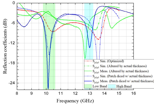
Fig. 10. Compared reflection coefficients of the fabricated samples.
