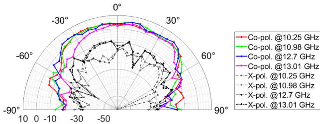
Fig. 12. Far-field radiation patterns of the realized gain at +45^\circ plane, when P1-port of the proposed antenna is ON.
