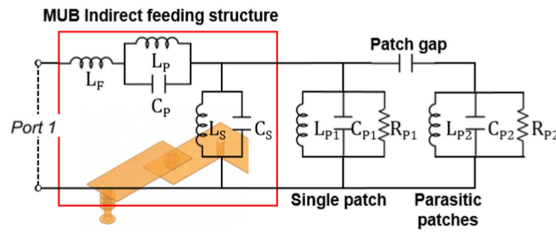
Fig. 5. Equivalent circuit model of MUB feeding structure. The component values are: L_F = 0.64 nH, L_P = 0.28 nH, C_P = 1.04 pF, L_S = 0.64 nH, and C_S = 0.24 pF.
