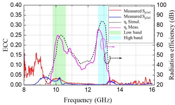
Fig. 11. ECC and radiation efficiency of a single antenna element along frequency, based on measured S_{p1N1} , S_{p2N1} , and simulated/measured efficiency.
