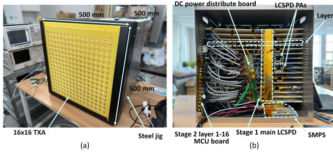
Fig. 9. Integrated 16 \times 16 TXA. (a) Front view. (b) Rearview.
