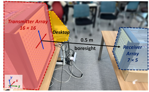
Fig. 15. Full-system configuration.
